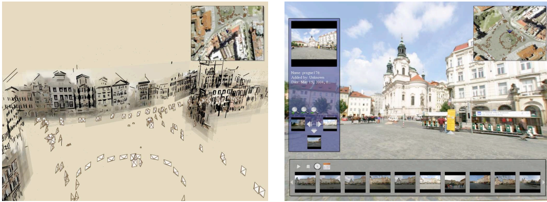
Figure 5: Screenshots from the explorer interface. Left: a view looking down on the Prague dataset, rendered in a non-photorealistic style. Right: when the user visits a photo, that photo appears at full-resolution, and information about it appears in a pane on the left.
